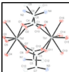
Fig. 1. View of the cation in (I) showing the atomic numbering and 50% probability displacement ellipsoids. H atoms have been omitted for clarity.
